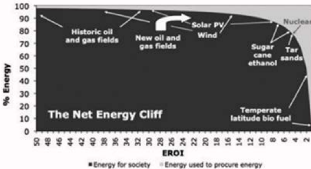
Figure 1. Net Energy Cliff, excerpted from Murphy et al. 2010. (21) Original figure legend: “The ‘Net Energy Cliff.’ As EROI approaches 1:1 the ratio of the energy gained (dark gray) to the energy used (light gray) from various energy sources decreases exponentially.”
